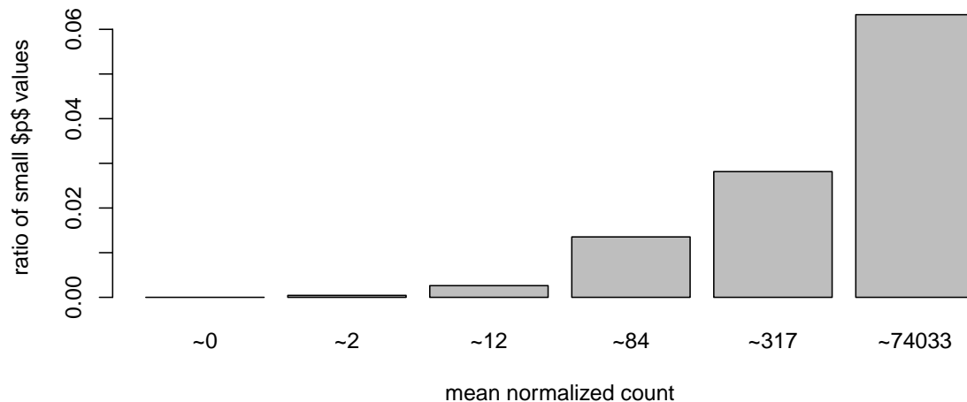
Figure 5: Ratio of small p values for groups of genes binned by mean normalized count
